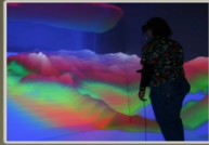
Cyberinfrastructure
