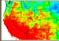
Climate Modeling
